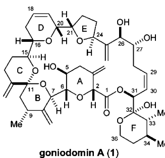
Figure 1. Structure of goniiodomin A
