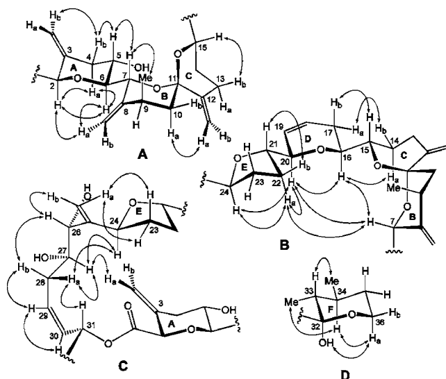
Figure 2. ROESY correlations for the C2–C15 (A), C7–C24 (B), C24–C31 (C), and C32–C36 (D) portions of goniiodomin A ( 1 ) (600 MHz, C 6 D 6 , acetone- d 6 , or CD 2 Cl 2 )
