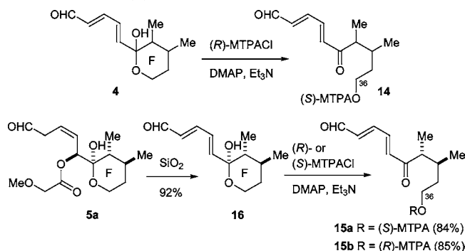
Scheme 3. Synthesis of ( S )-MTPA Ester 14 and ( S )- and ( R )-MTPA Esters 15a and 15b
