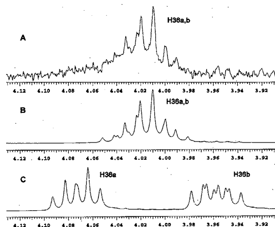
Figure 3. Partial ^1\text{H} NMR spectra (600 MHz, \text{C}_6\text{D}_6 ) of ( S )-MTPA ester 14 (A), ( S )-MTPA ester 15a (B), and ( R )-MTPA ester 15b (C).
